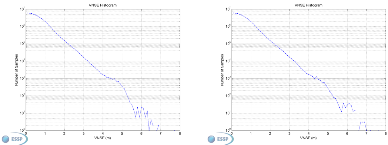
Figure 5 – EGNOS APV-I Vertical Navigation System Error: PRN 120 (left) and PRN124 (right)
