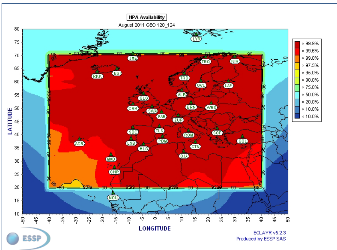
Figure 8 - EGNOS NPA Availability
