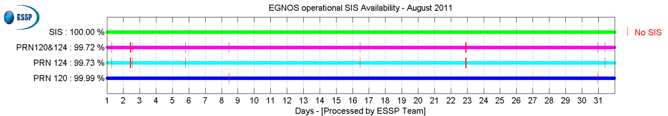
Figure 1 – EGNOS SIS & PRN Availability for August 2011(%)
