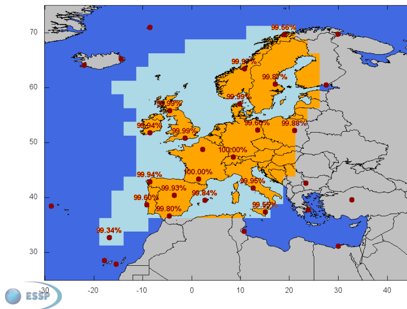
Figure 7 - EGNOS Open Service Availability at reference stations (PRN124)
