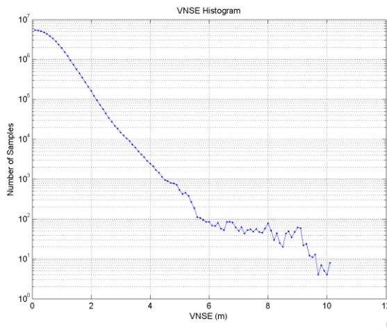
Figure 14 – EGNOS APV-I Vertical Navigation System Error: PRN 120 (left) and PRN124 (right).
