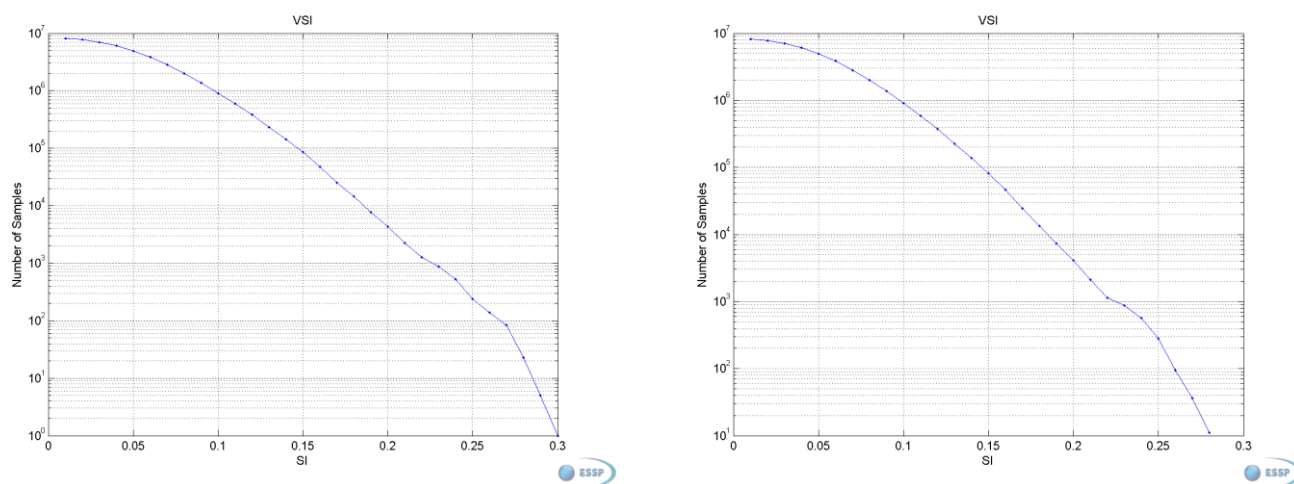
Figure 12 – EGNOS APV-I Vertical Safety Index of the month: PRN 120 (left) and PRN124 (right).
