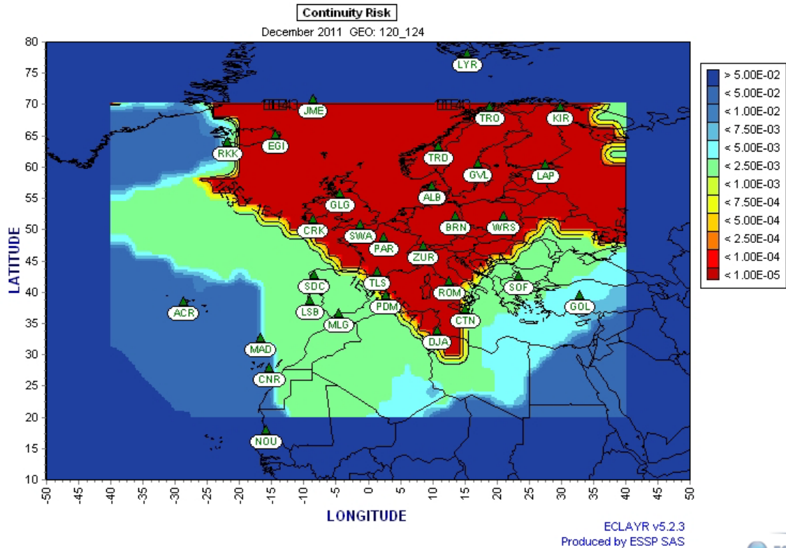
Figure 7 - EGNOS NPA Continuity.
