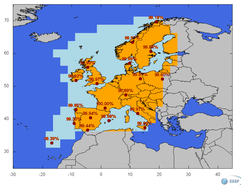
Figure 5 - EGNOS Open Service Availability at reference stations (PRN124).
