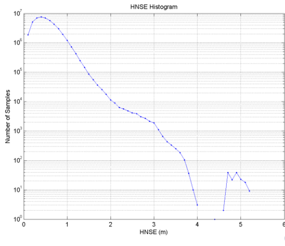
Figure 13 – EGNOS APV-I Horizontal Navigation System Error: PRN 120 (left) and PRN124 (right).
