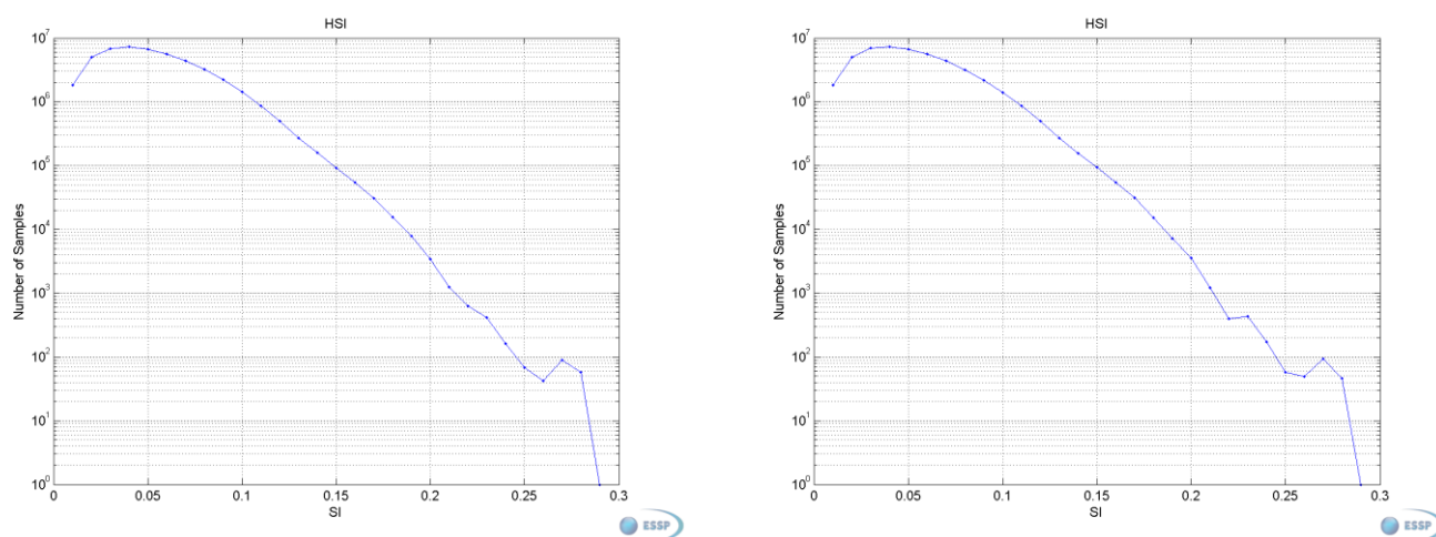
Figure 11 – EGNOS APV-I Horizontal Safety Index of the month: PRN 120 (left) and PRN124 (right).
