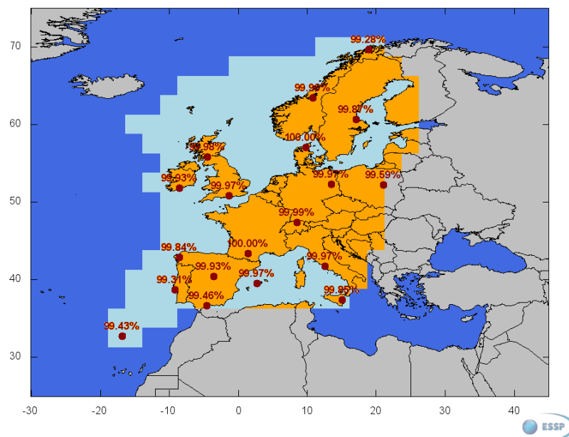
Figure 4 – EGNOS Open Service Availability at reference stations (PRN120).
