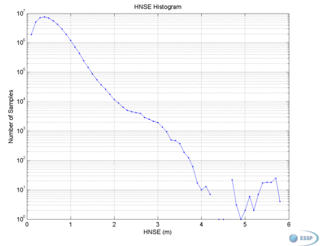
Figure 13 – EGNOS APV-I Horizontal Navigation System Error: PRN 120 (left) and PRN124 (right).
