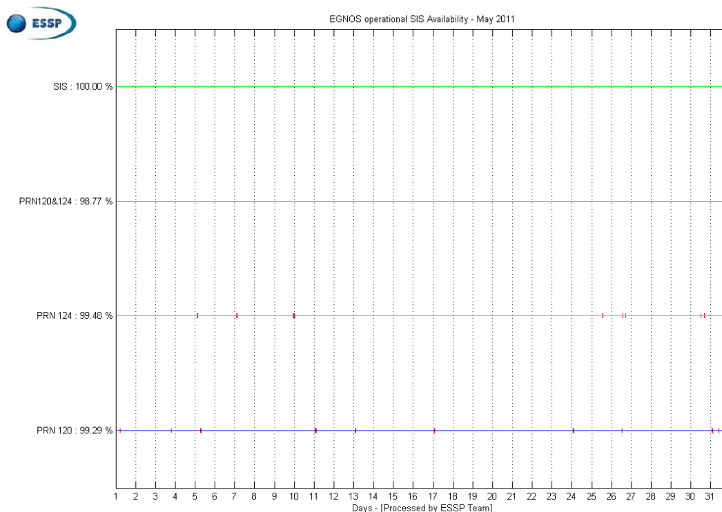
Figure 1 – EGNOS SIS & PRN Availability for May 2011(%)
