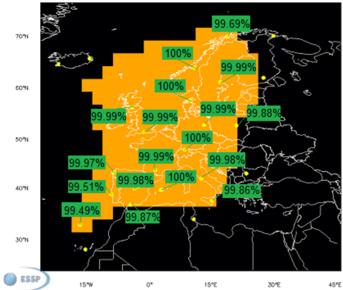
Figure 5 - EGNOS Open Service Availability at reference stations at reference stations (PRN124)
