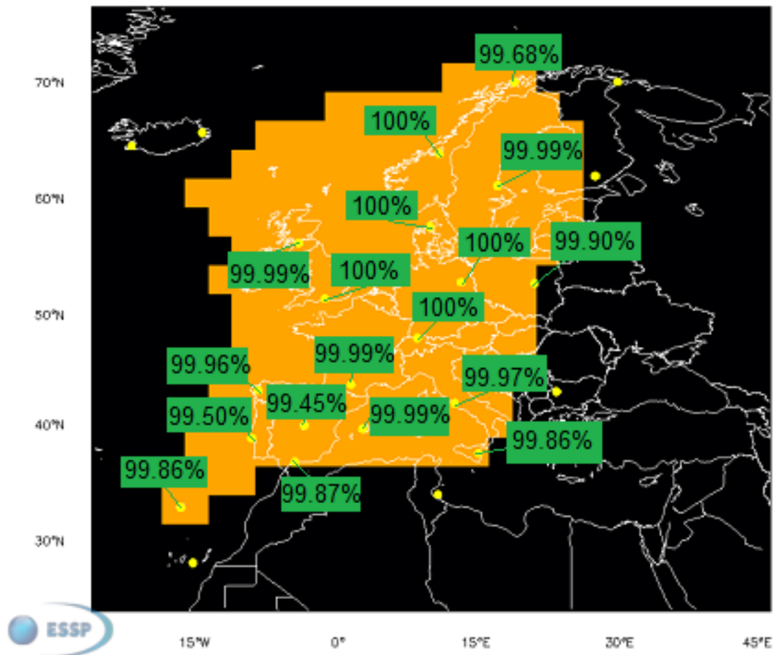
Figure 4 – EGNOS Open Service Availability at reference stations (PRN120)
