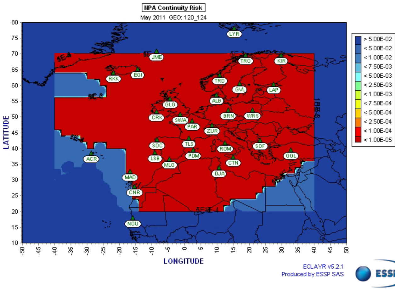
Figure 7 - EGNOS NPA Continuity
