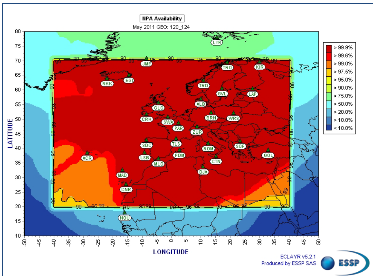
Figure 6 - EGNOS NPA Availability
