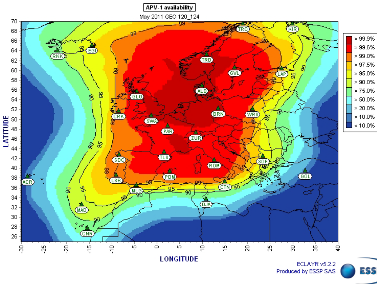
Figure 8 – EGNOS APV-I Availability
