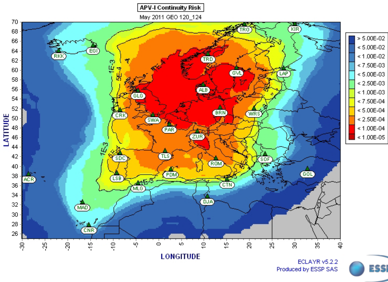
Figure 9 – EGNOS APV-I Continuity
