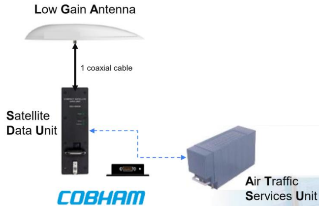
Figure 5-1: FANS-C over SatCom Avionics
