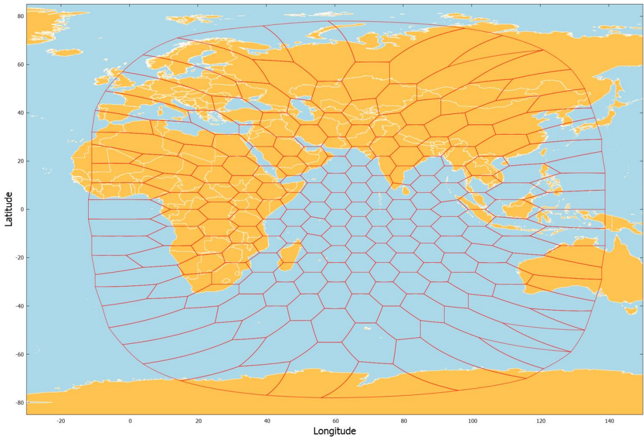
Figure 4-6: MEAS narrow spot beams 12
