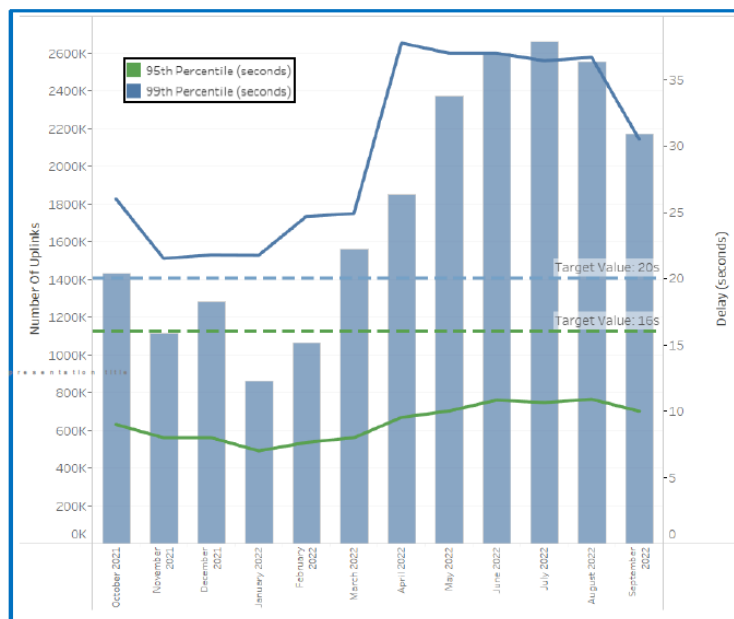
Figure 7-1: Technical Round Trip Delay (TRTD) for ATN/VDLM2 based services
