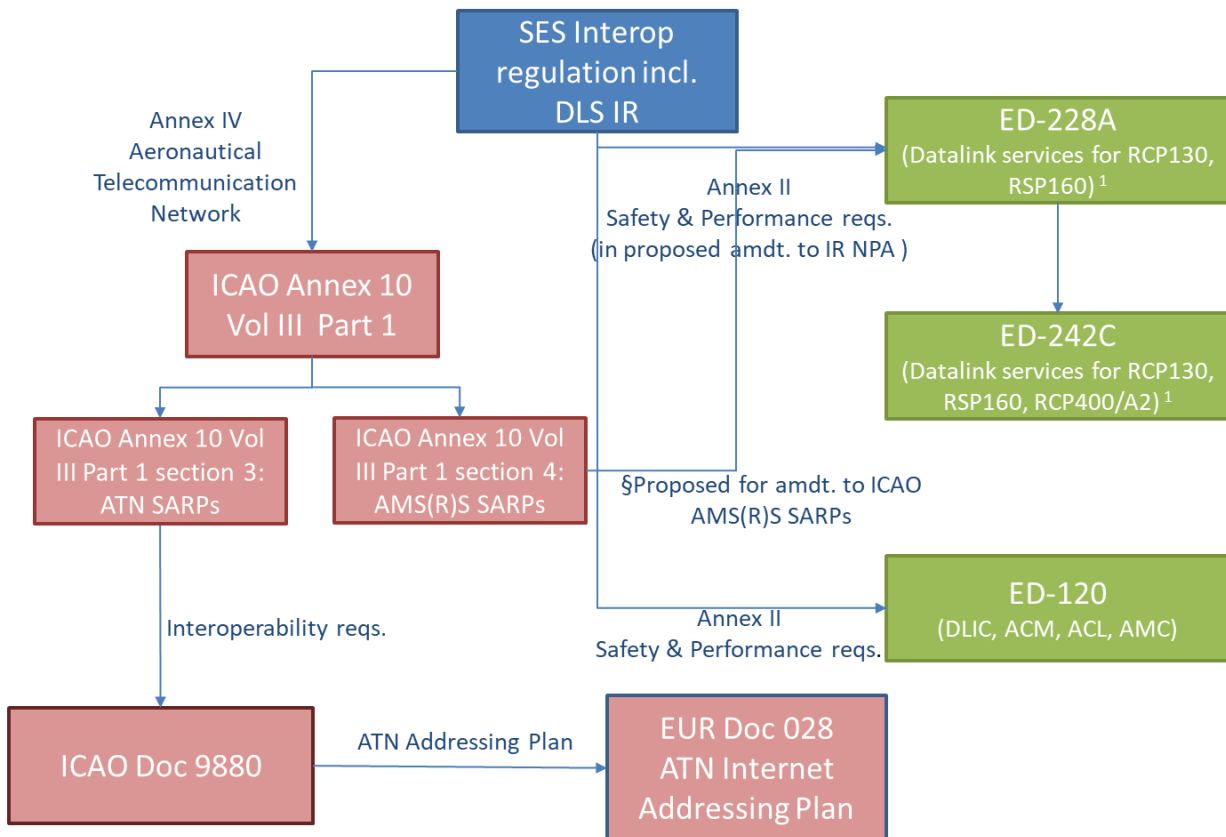
Figure 3-1: Schematic of the DLS IR and applicable standards
