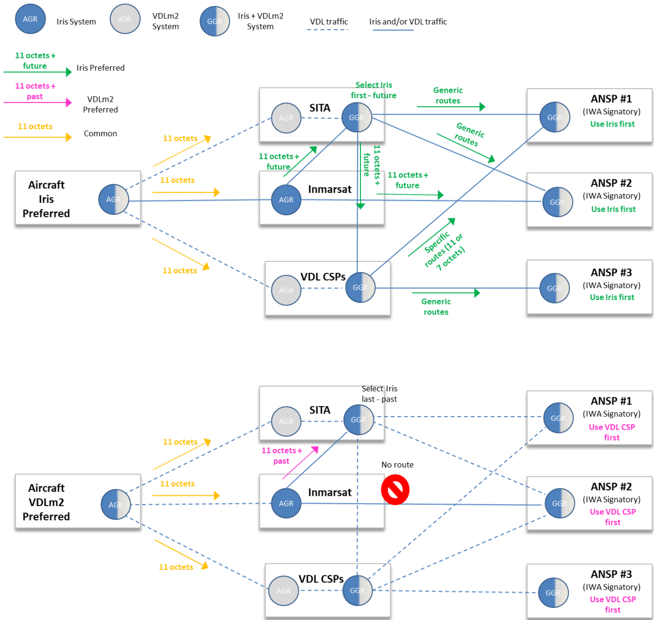
Figure 4-3 ATN/OSI Multilink - Link Preference Signalling
