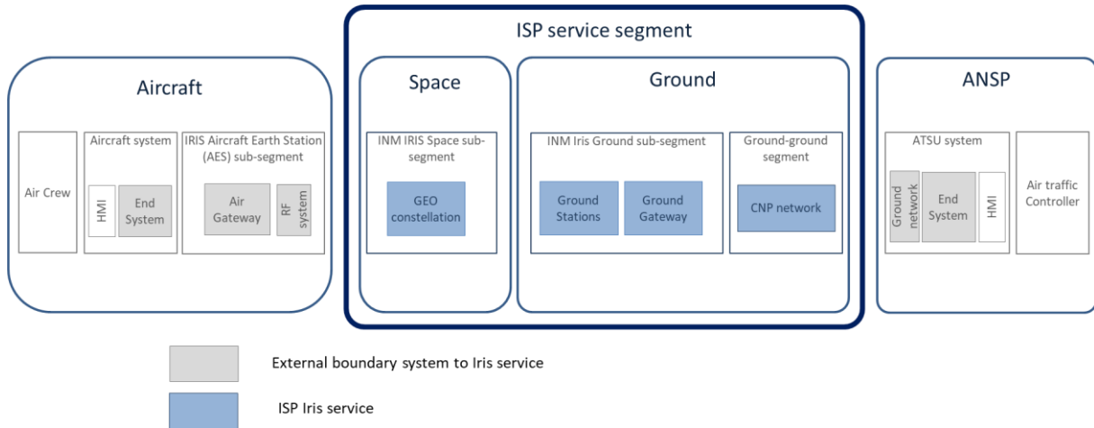
Figure 4-1: Iris System Architecture
