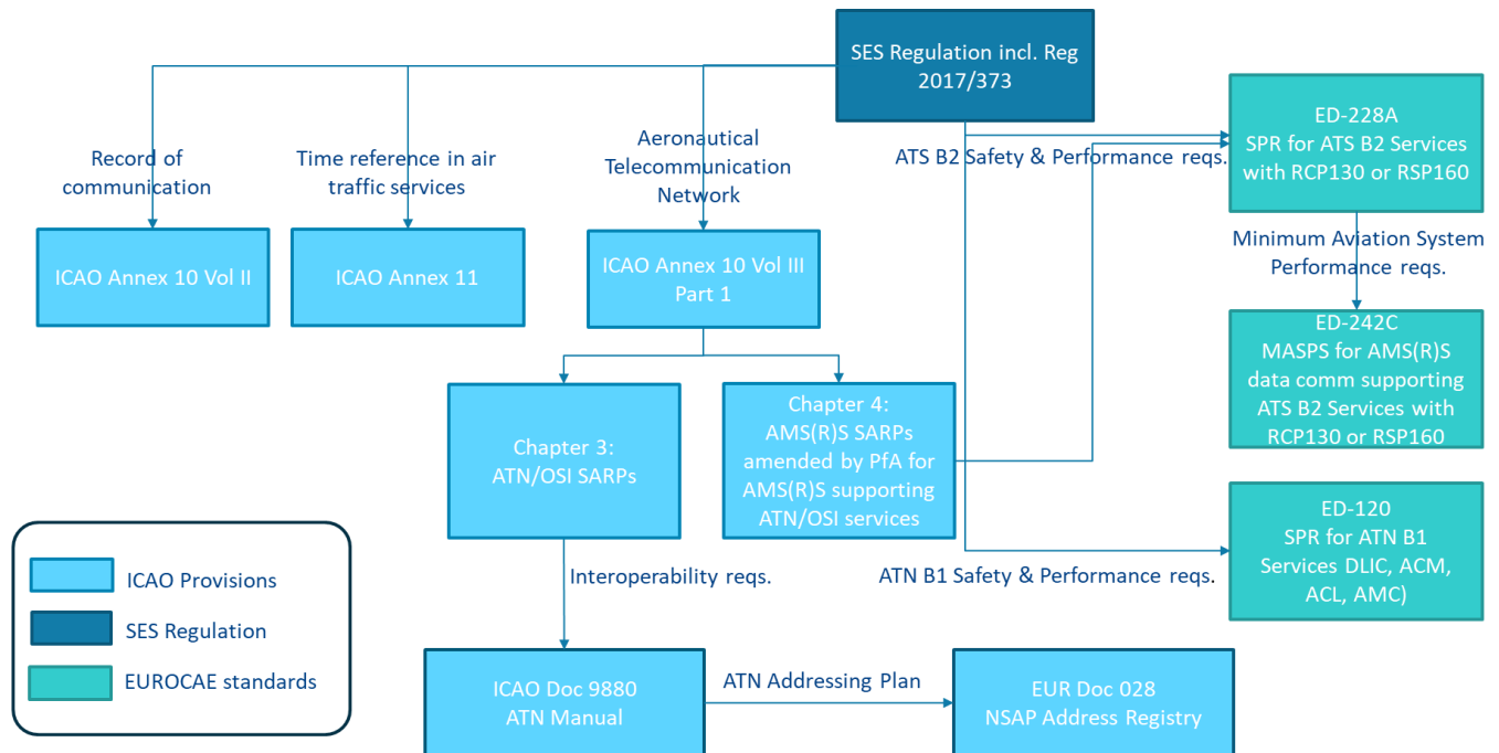
Figure 3-1: Schematic of the applicable regulatory provisions and applicable standards
