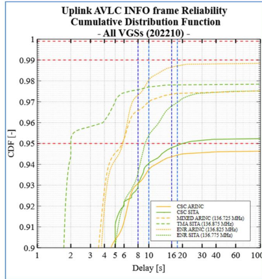
Figure 7-3: AVL reliability
