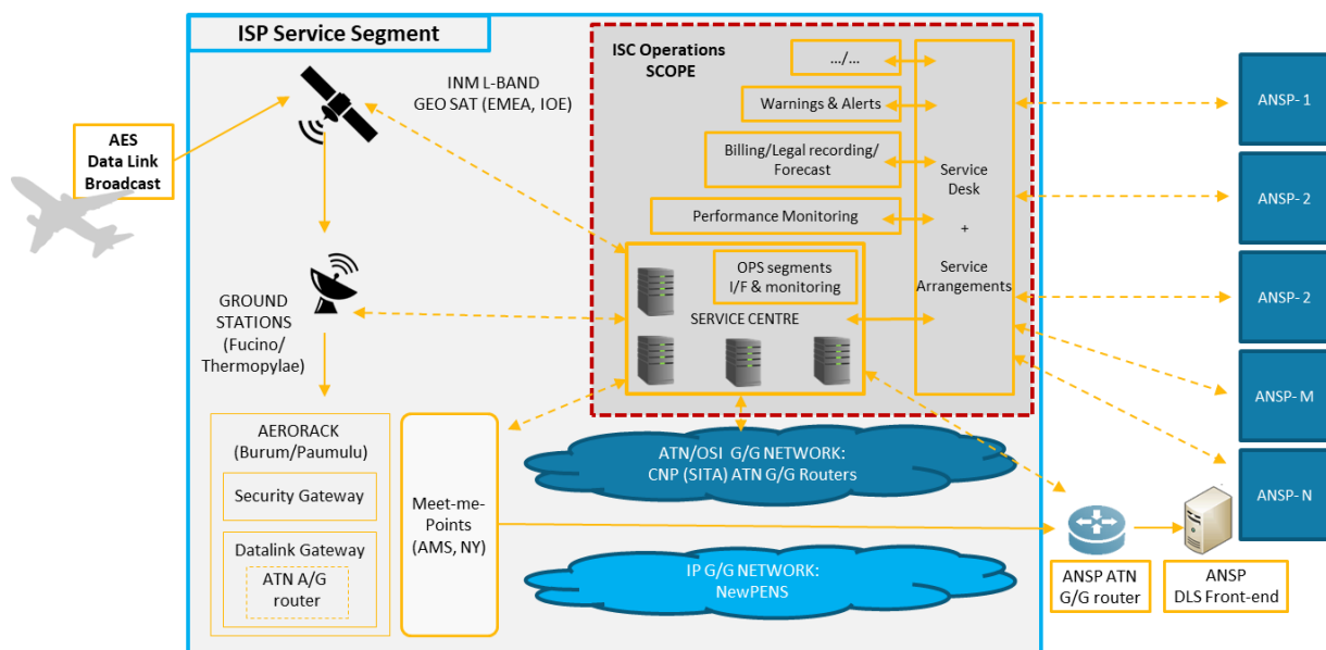
Figure 4-2: ISP Service Center (ISC)
